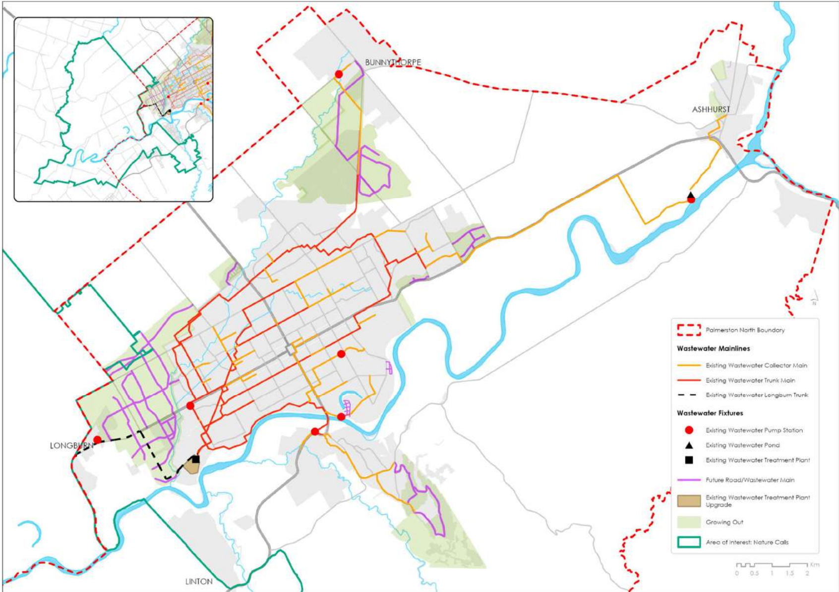
Map 11: Wastewater network
